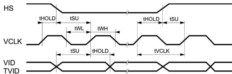
Figure 4. Setup and Hold Timing.
